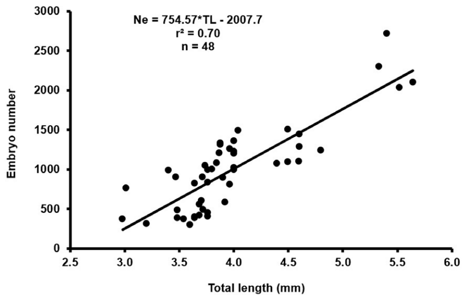
Figure 4. Relationship between numbers of embryos ( Ne ) and total length ( TL ) in Probopyrus pandalicola ovigerous females with embryos in stage I of development.
