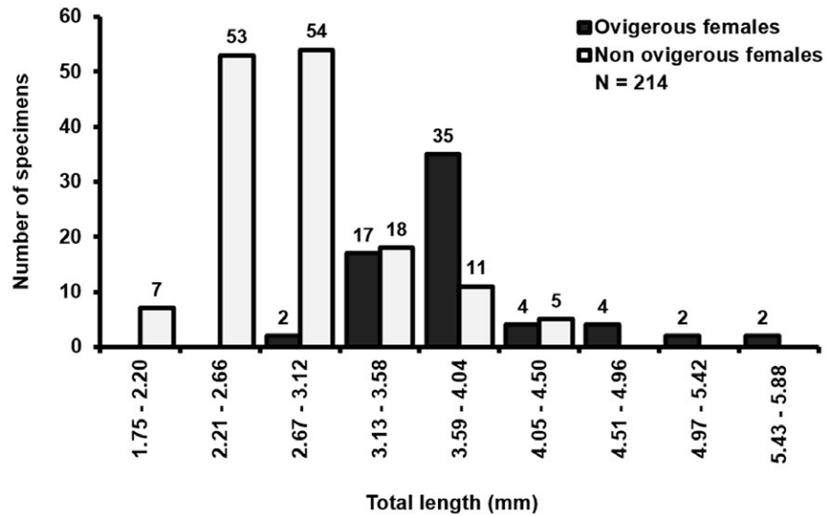
Figure 3. Size-frequency distribution of Probopyrus pandalicola non-ovigerous females and ovigerous females. The number of individuals is shown above each size-class bars.
