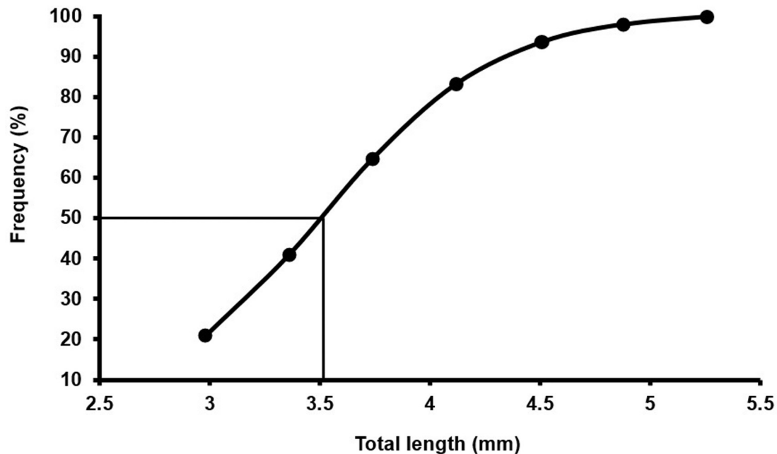
Figure 5. Logistic function between the proportion and total length (TL) of Probopyrus pandalicola ovigerous females. TL50 corresponds to 50% of the size at functional sexual maturity.
