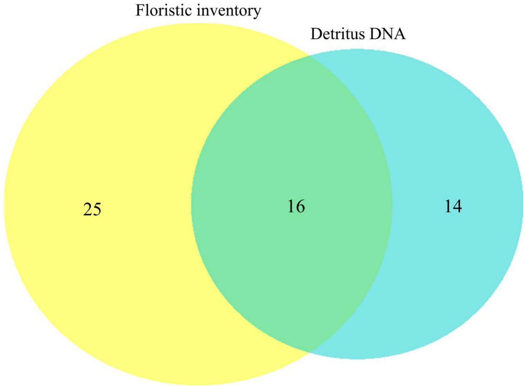
Supplementary Fig. 1. Venn diagram of the similarity between the floristic inventory (to the left), debris as detected by DNA (to the right), and family-shared taxa in the center.
